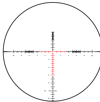
SCR Reticle
