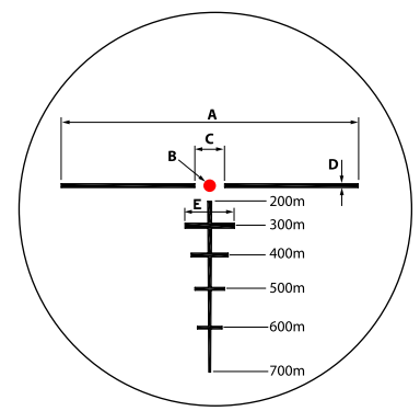
RAPID DOT 5.56, 7.62 RETICLE SUBTENSION
